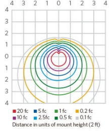
TD 6LED ISOFOOTCANDLE PLOT
